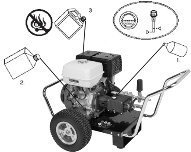
FIGURE 2.1 - CHECK MACHINE
