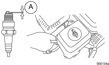
Figura 4-13. Bujía
