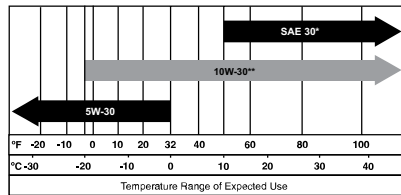
Figure 4-9. Oil Viscosity
