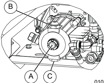
Figure 4-6. Drain/Fill Oil
