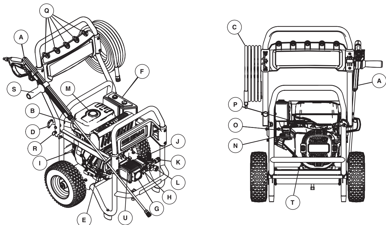
Figure 1 – Features & Controls
