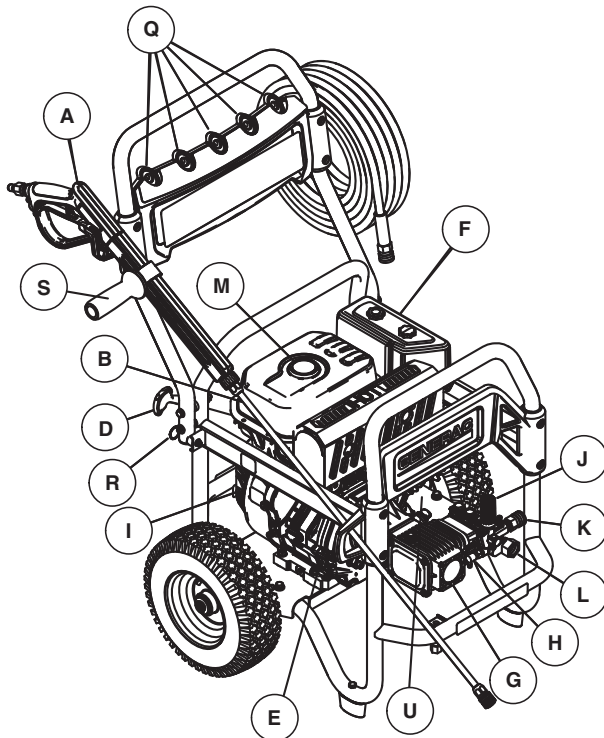
Figure 1 – Features & Controls
