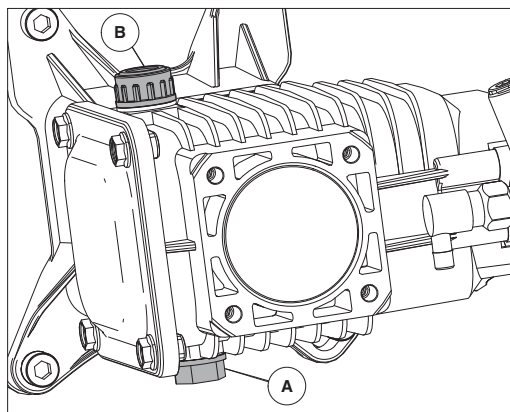
Figure 34 – Dipstick
