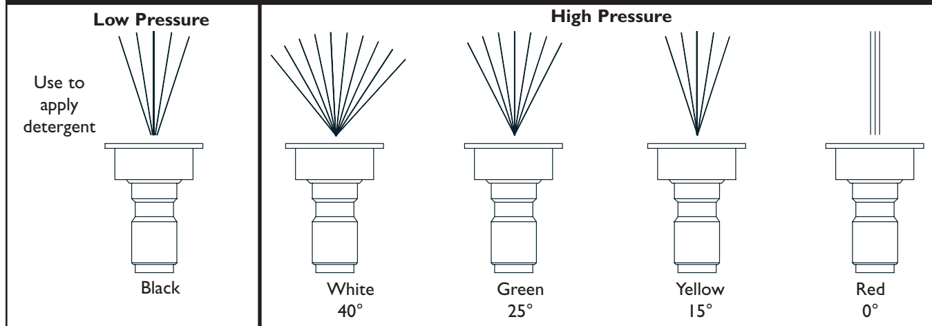
Figure 11 — Spray Tips
